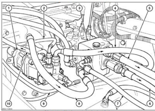
Oil pump and loader control valve installation
